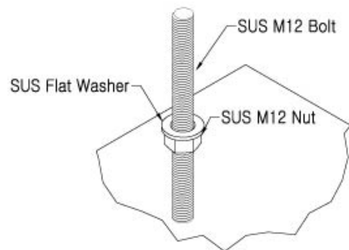
"A" Detail
