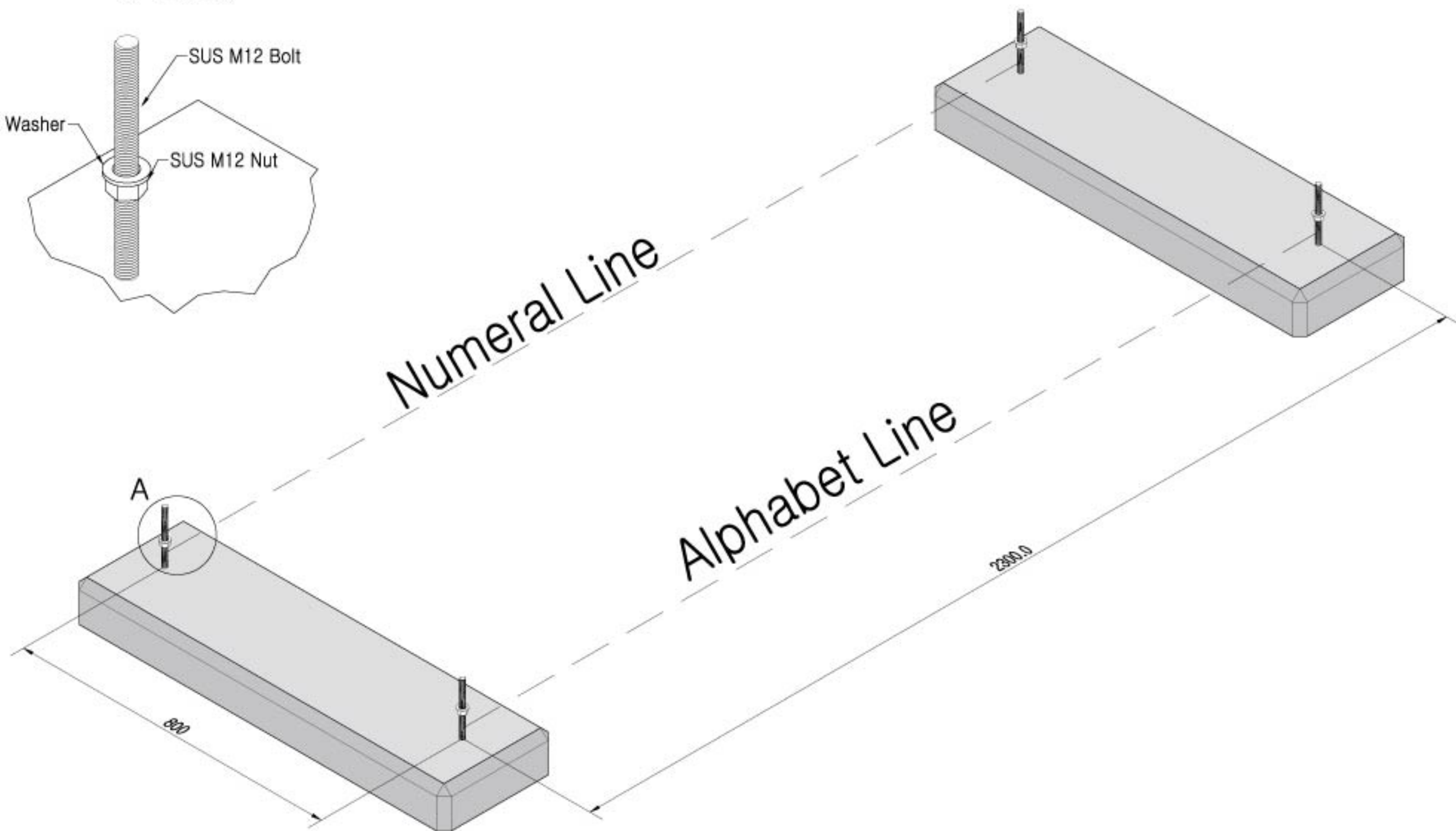
"A" Detail
