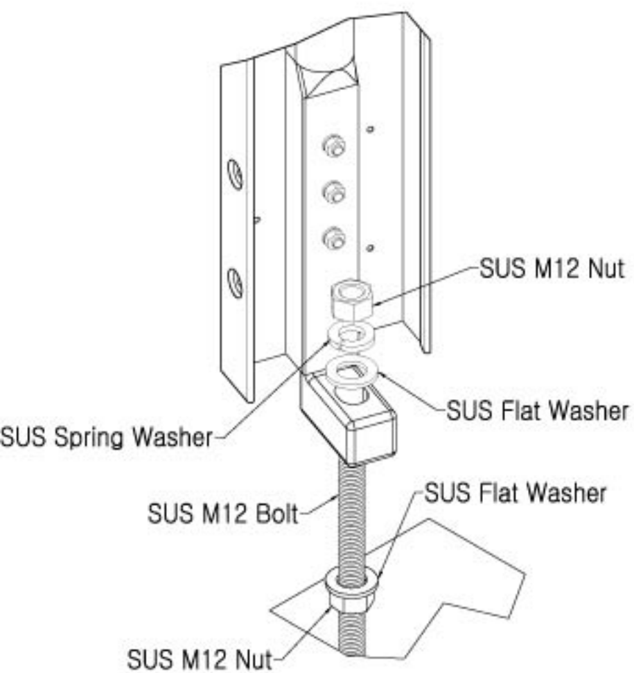
"B" Detail
